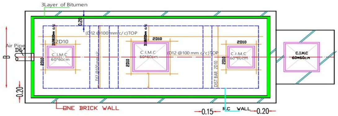
SEPTIC TANK COVER PLAN
